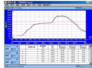
( The Profiles Are Detected by "THERMOTRACKER" Model : PRO-1000 )
